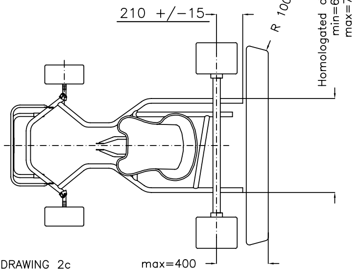
DRAWING 2c REAR PROTECTION 2006
